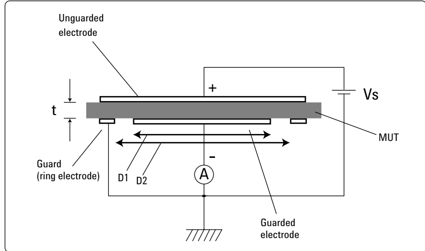
Figure 35. Volume resistivity
